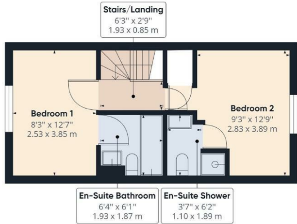
Floor 1 Building 1
